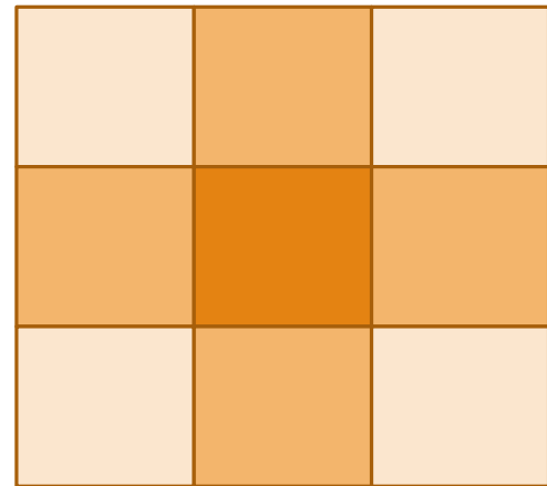
3 x 3 image
