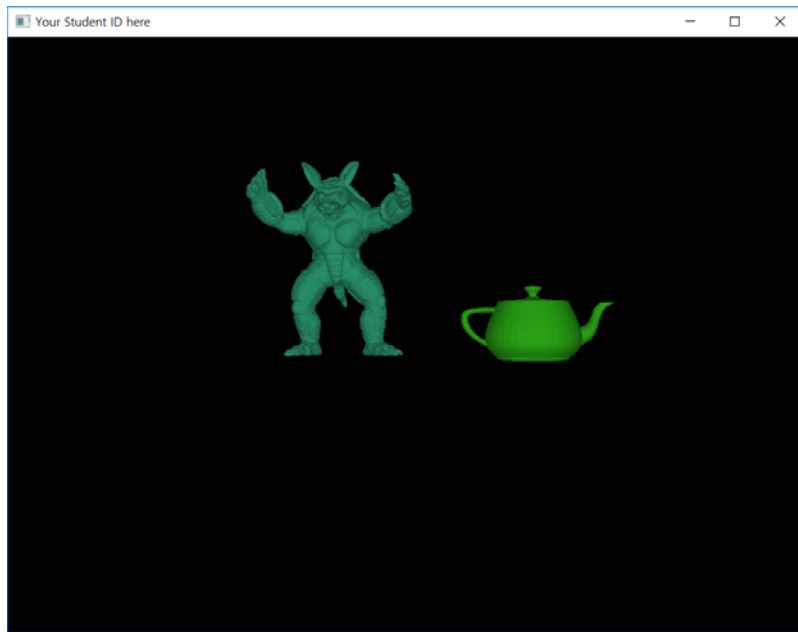
Front buffer
