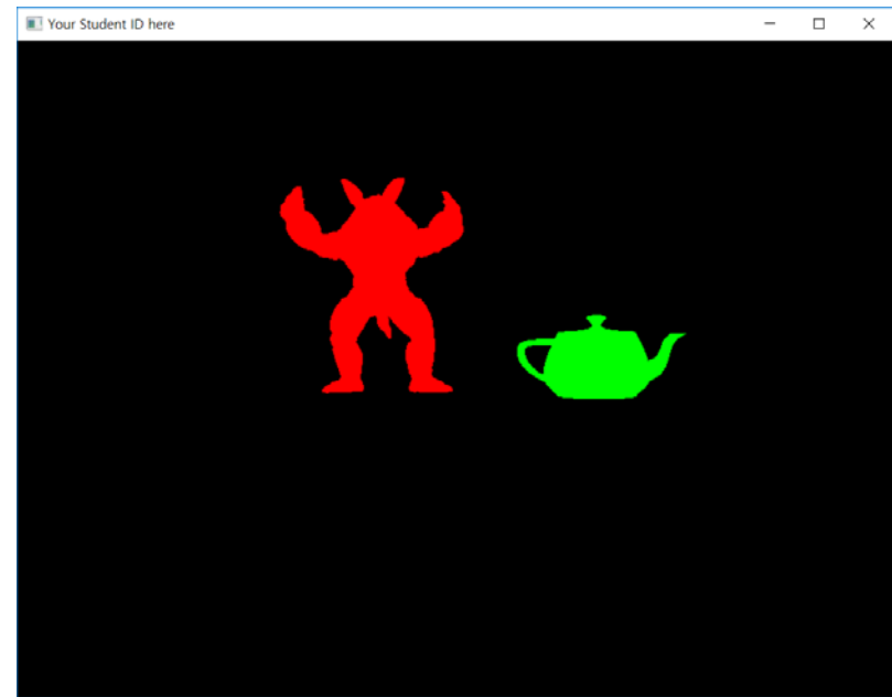
Back buffer
